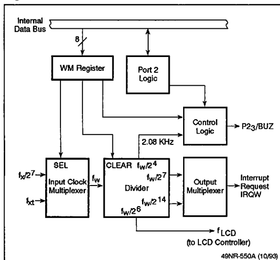
Figure 10. Watch Timer
