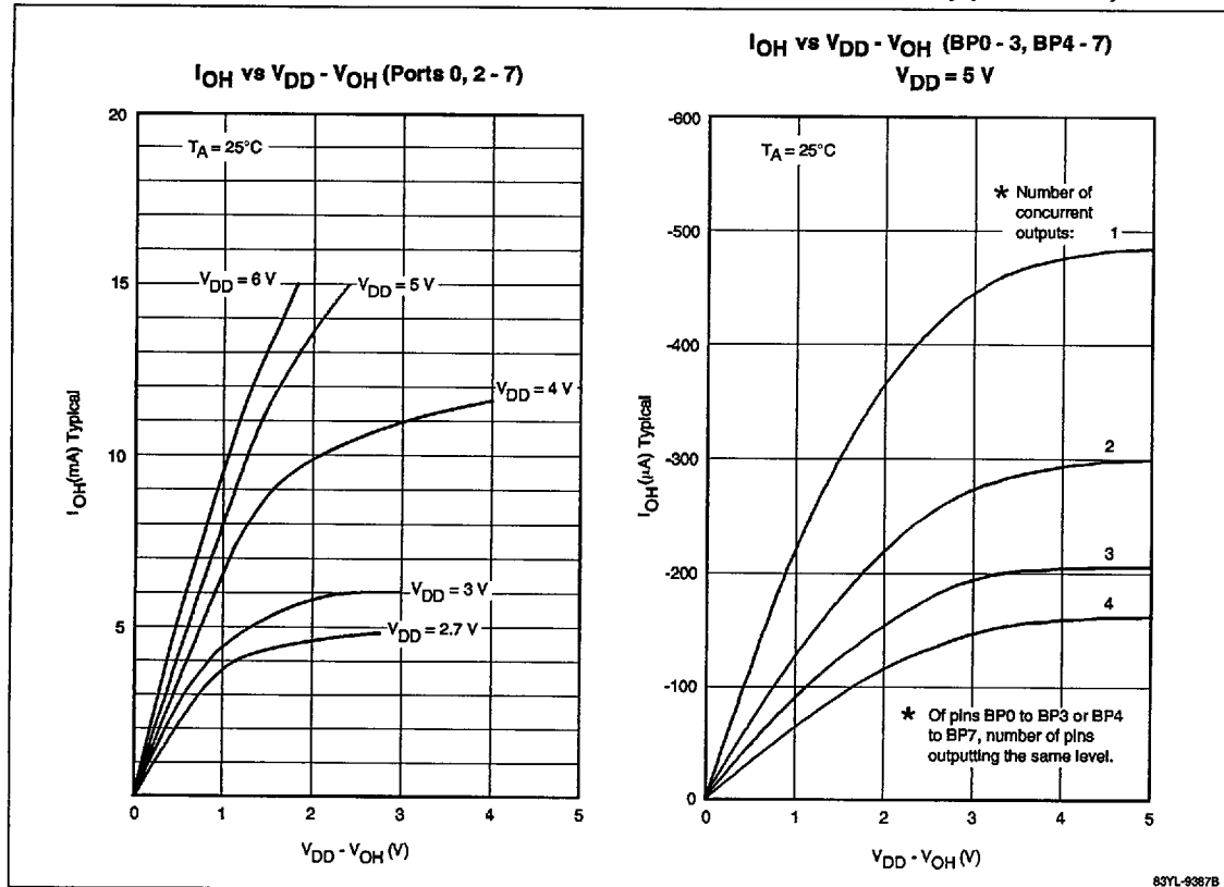
Figure 21. DC Characteristics, I_{OH} vs V_{DD} - V_{OH} (μPD7530x/31x, Standard Grade) (Sheet 1 of 2)
