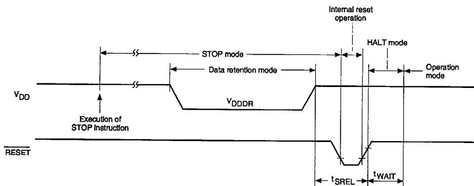
Figure 29. Low-Voltage Data Retention Timing
